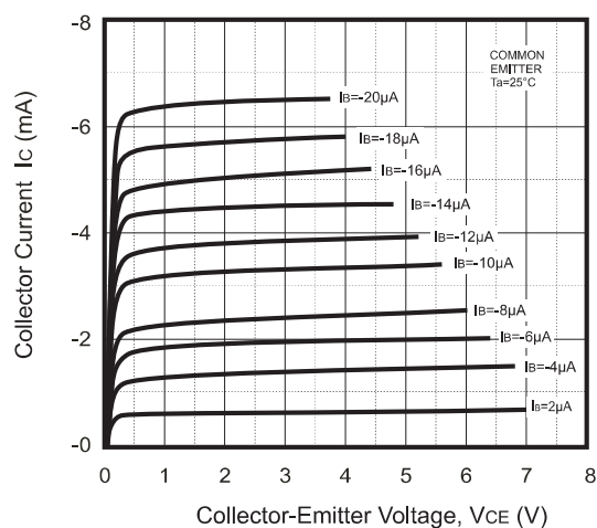
Fig.1 - Static Characteristic
